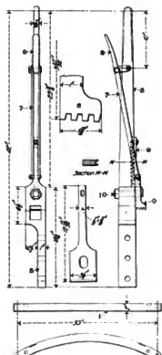
Figs. 1952-1958. Reverse Lever and Quadrant.
